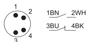
Fig. 9 1 NO + 1 NC (without LED)
